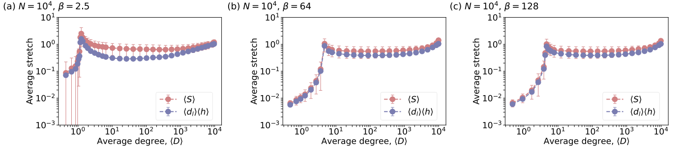
FIG. F1: Comparison of the average stretch and the product of the average link length and average hopcount as functions of the average degree for SRGG networks with N = 10^4 nodes, for different values of \beta . The average stretch is computed over 10^6 randomly selected node pairs, and the error bars indicate standard deviations.
