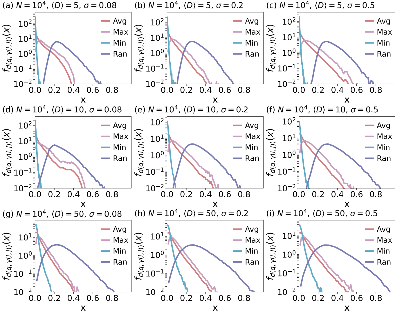
FIG. B5: The distribution of the average (avg), maximum (max), and minimum (min) distances between shortest path nodes and geodesics connecting shortest path endpoints in SRGGs where nodes are not uniformly scattered and the connection probability function is given by Eq. (5). The distribution of distances to geodesic from randomly selected nodes (ran) are also presented. The network size N = 10^4 . For each average degree \langle D \rangle and standard deviation \sigma of the Gaussian distribution used to sample node coordinates, we generated an SRGG and considered 10^6 random shortest paths.
