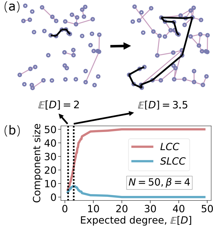
FIG. C1: (a) Visualizations of toy SRGGs with N = 50 nodes and inverse temperature \beta = 4 for increasing expected degree, from left to right: \mathbb{E}[D] = 2 , \mathbb{E}[D] = 3.5 . In each graph, a representative shortest path is highlighted in black. (b) Average sizes of the largest connected component (LCC) and the second largest connected component (SLCC) for SRGGs with N = 50 and \beta = 4 as a function of the expected degree \mathbb{E}[D] . The emergence of a giant connected component occurs at the critical expected degree D_c = 3.5 , identified by the maximum of the SLCC. All LCC and SLCC values are averaged over 100 independent realizations. Accordingly, the graph visualizations in panel (a) correspond to the disconnected and critical connected regimes.
