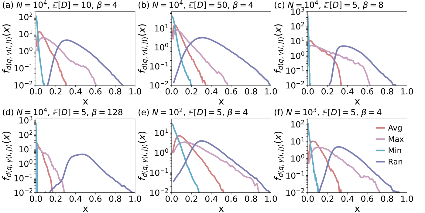
FIG. B1: The distribution of the average (avg), maximum (max), and minimum (min) distances between shortest path nodes and geodesics connecting shortest path endpoints. For comparison, we also plot the distribution of distances to geodesic from randomly selected nodes (ran). The distributions in (a)-(d) are obtained for a single SRGG realization and 10^6 random shortest paths. For panels (e) and (f), we generated 10^3 SRGG realizations. For each G_i , i = 1, \dots, 10^3 , we considered 10^3 random shortest paths.
