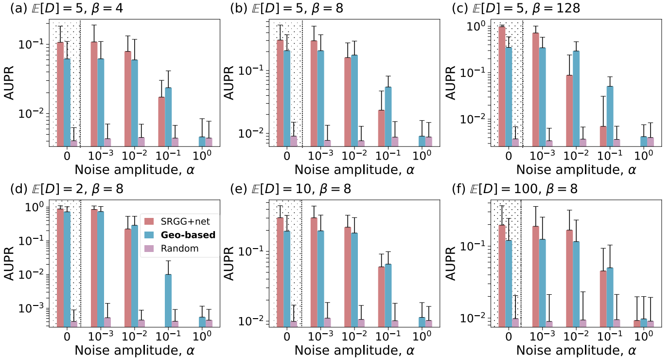
FIG. E1: AUPR of shortest-path identification using the distance to geodesic (geometry-based) method. Panels show the average AUPR as a function of the coordinate noise amplitude \alpha , for different combinations of \mathbb{E}[D] and \beta . All experiments are performed on SRGG networks with N = 10^4 nodes. Each bar represents the average AUPR over 10^2 randomly selected node pairs and the error bars indicate standard deviations.
