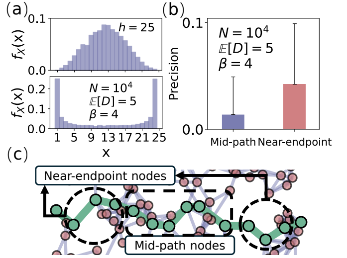
FIG. 7: (a, top) The distribution of shortest path node positions with the largest distance to geodesic. (a, bottom) The distribution of shortest path node positions with the smallest distance to geodesic. In both distributions, we consider shortest paths of fixed hopcount, h = 25 , and SRGGs with N = 10^4 nodes, inverse temperature \beta = 4 , and the expected degree \mathbb{E}[D] = 5 . The most remote from the geodesic nodes are likely to be found in the middle of a shortest path, while the closest to the geodesic nodes are likely to be found close to the path endpoints. See Appendix B for plots with other SRGG parameters. (b) The precision of finding shortest path nodes near endpoints (Near-endpoint) and in the middle of the path (Mid-path) using the distance to the geodesic. A 10^4 -node SRGG is generated. Each bar is the average precision computed for 100 randomly selected node pairs and the error bars depict standard deviations. (c) shows an example illustrating the division of Near-endpoint nodes and Mid-path nodes on a shortest path.
