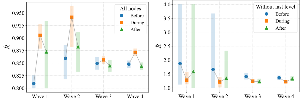
Fig 12. Average outdegree and 95% confidence intervals for the infection trees belonging to different periods around the peak of the four COVID-19 waves in Cyprus. The trees are divided into three groups: trees whose nodes were only tested positive before the peak (Before), trees whose nodes were tested positive before and after the peak (During), and trees whose nodes were only tested positive after the peak (After). On the left the plot when no pruning is applied. On the right the estimate where the last level of the infection trees is pruned.
