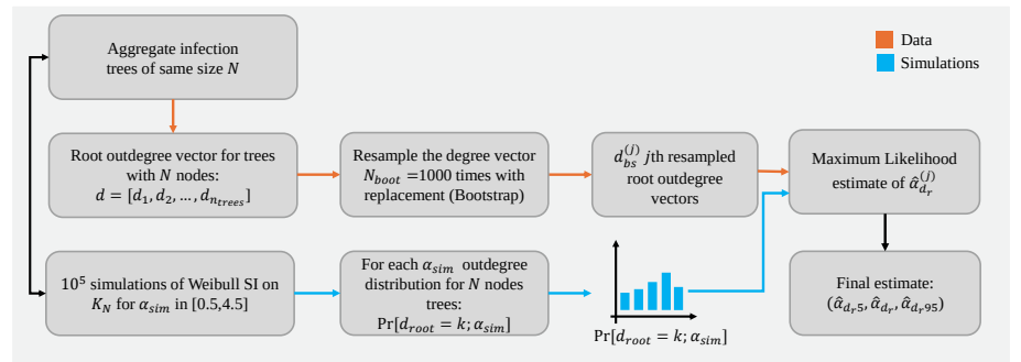
Fig 5. Flow chart of Method 2 based on root outdegree distribution, details in S4 Appendix.
