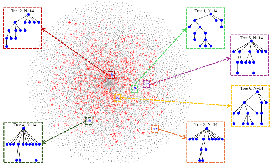
Fig 1. Infection trees of the fourth wave (April 2021 - May 2021) of COVID-19 epidemic in Cyprus. The zoomed in view displays a subset of the infection trees of size N = 14 . Trees with less than 5 nodes are shown in gray, while larger trees (5 or more nodes) are shown in red.
