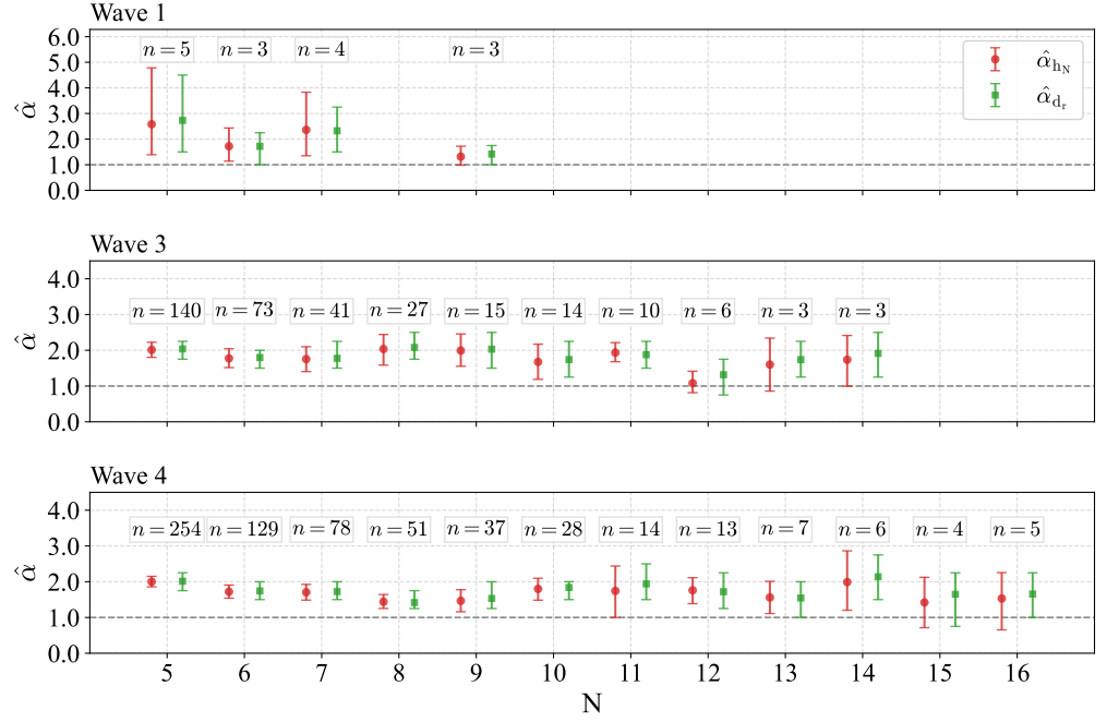
Fig 8. Summary of all the results obtained on the sets of infection trees of wave 1, 3 and 4. In red the estimates of the shape parameter \alpha employing the method based on the hopcount distribution of the infection trees ( \hat{\alpha}_{hN} ). In green, the estimates of the shape parameter \alpha employing the method based on the root outdegree distribution of the infection trees ( \hat{\alpha}_{dr} ). The error bars represent the 90 % confidence intervals given by the bootstrap procedure performed resampling 1000 times with replacement each set of trees of the same size. The number n on top of each estimate indicates how many infection trees are employed for a given size N .
