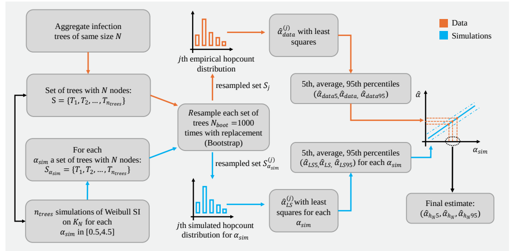
Fig 4. Flow chart of Method 1 based on hopcount distribution, details in S4 Appendix.
