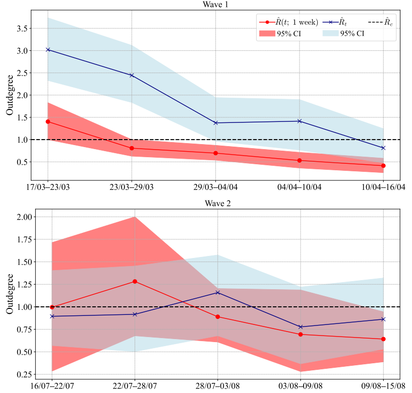
Fig 11. Evolution of the effective reproduction number \hat{R}(t; 1 \text{ week}) in the first two waves of the COVID-19 epidemic in Cyprus. The red line shows the mean outdegree for each week derived from bootstrapped samples, with the 95% confidence intervals indicated as a red area. The blue line for Wave 1 represents the effective reproduction number reported in Fig. 10 of [42]. The blue line for Wave 2 displays values from [44]. In dashed black the reference line at the critical value \hat{R}_c = 1 .
