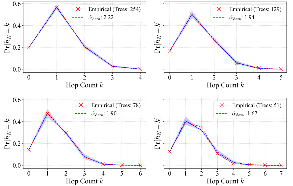
Fig 6. Hopcount distribution for infection trees belonging to wave 4 of size N = 5, 6, 7, 8 . Red line: empirical hopcount distribution obtained aggregating trees of the same size N . Dashed blue line: distribution (7) with parameter \hat{\alpha}_{\text{data}} , which corresponds to the average of the least squares estimates \hat{\alpha}_{\text{data}}^{(j)} , j = 1, \dots, 1000 . The blue area spans the distributions (7) with shape parameter \alpha in the 90% confidence intervals of the least square estimate \hat{\alpha}_{\text{data}} .
