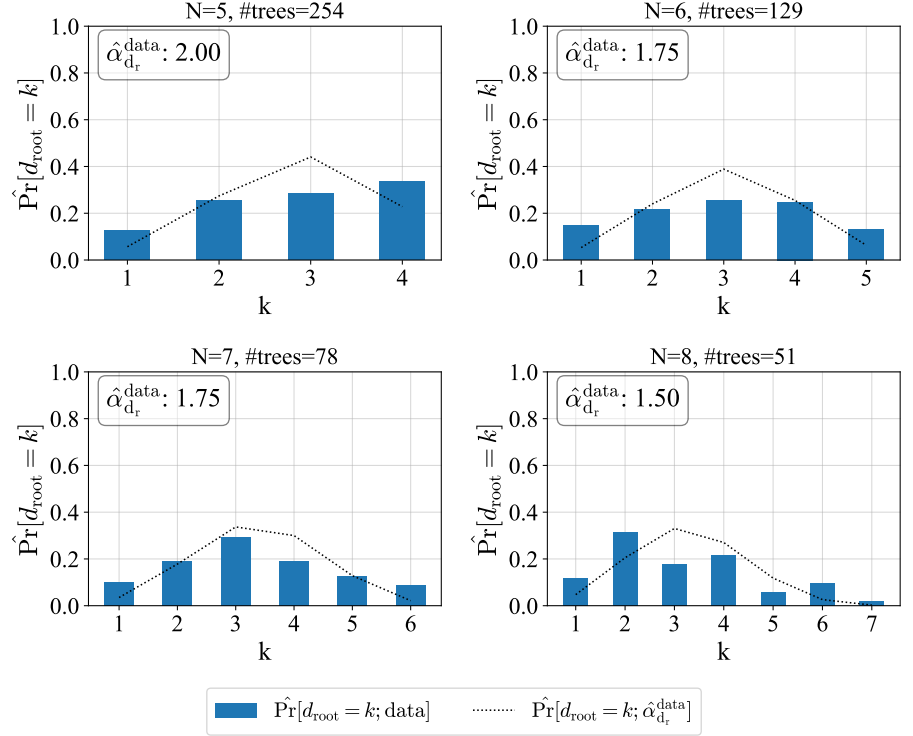
Fig 7. Empirical root outdegree distribution obtained from the set of infection trees of size N = 5, 6, 7, 8 belonging to wave 4. In black the root outdegree distribution obtained from the non-Markovian SI simulation on the complete graph with size N and \alpha_{\text{sim}} equal to the maximum likelihood estimate \hat{\alpha}_{\text{d}_r}^{\text{data}} in the range [0.5, 4.5] (with steps of 0.25) given the empirical distribution. In blue the empirical root outdegree distribution.
