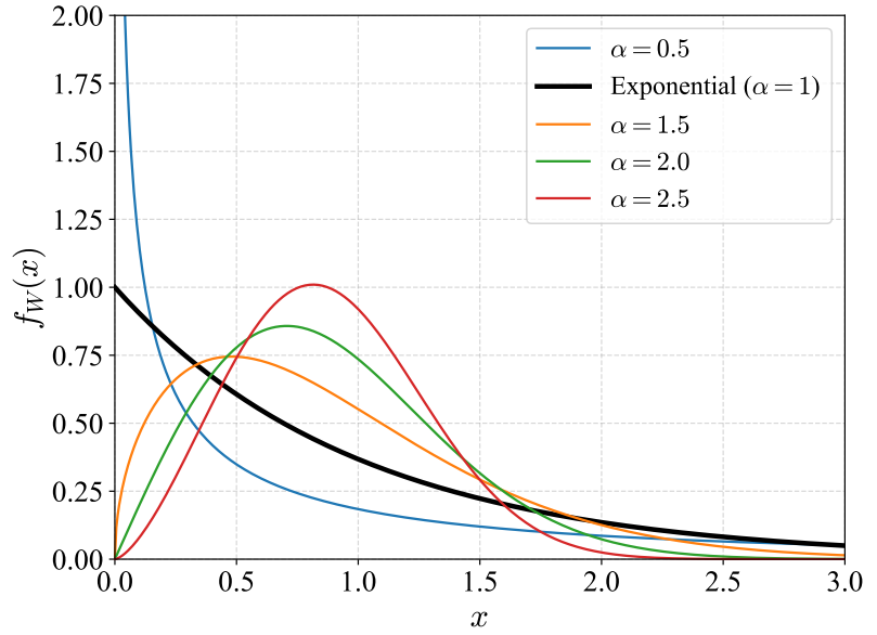
Fig 3. The Weibull probability density function (6) with rate parameter \beta equal to 1 and different shape parameters 0.5 \leq \alpha \leq 2.5 .
