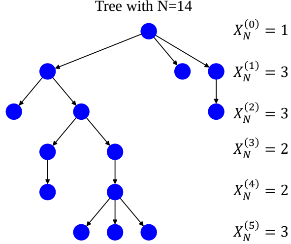
Fig 2. An real infection tree with N = 14 nodes. The variables X_N^{(h)} represent the number of nodes located exactly at h hops from the root. For instance, at hopcount h = 1 , there are X_{14}^{(1)} = 3 nodes.
