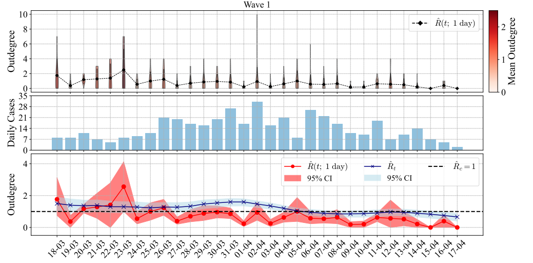
Fig 9. Daily out-degree distribution (top) and daily reported case counts (middle) during the first COVID-19 wave in Cyprus. Violin plots represent the distribution of secondary infections per case per day; color intensity indicates the mean outdegree. (Bottom) Evolution of the effective reproduction number \hat{R}(t; 1 \text{ day}) in the first wave of the COVID-19 epidemic in Cyprus. The red line shows the mean outdegree for each day derived from bootstrapped samples, with the 95% confidence intervals indicated by the red area. The blue line represents the effective reproduction number reported in [44]. In dashed black the reference line at the critical value \hat{R}_c = 1 .
