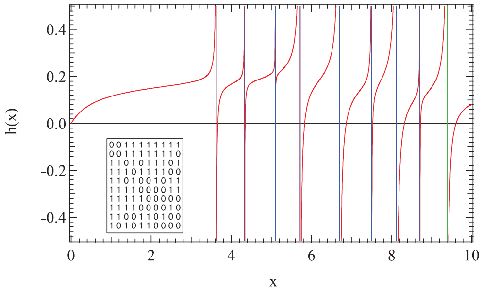
Figure 1. The function h(x) in (76) versus x for an instance of an Erdos-Renyi random graph G_p(N) with link density p on N = 10 nodes, specified by the shown adjacency matrix in the rectangle with zero-one entries. The vertical asymptotes are shown in blue; only the largest vertical asymptote is drawn in green.
