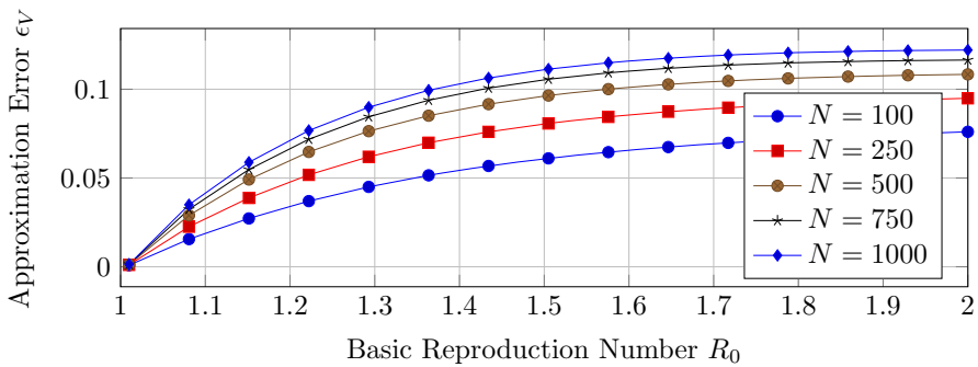
(b) Barabási-Albert random graphs.
