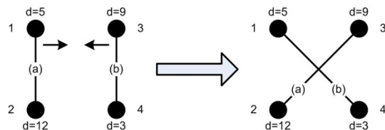
Figure 13: degree-preserving rewiring
