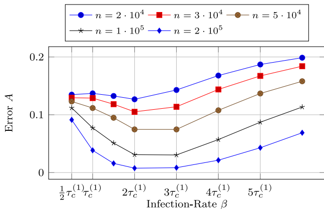
Fig. 8. Average error of estimates of A in dependency of the infection rate \beta .
