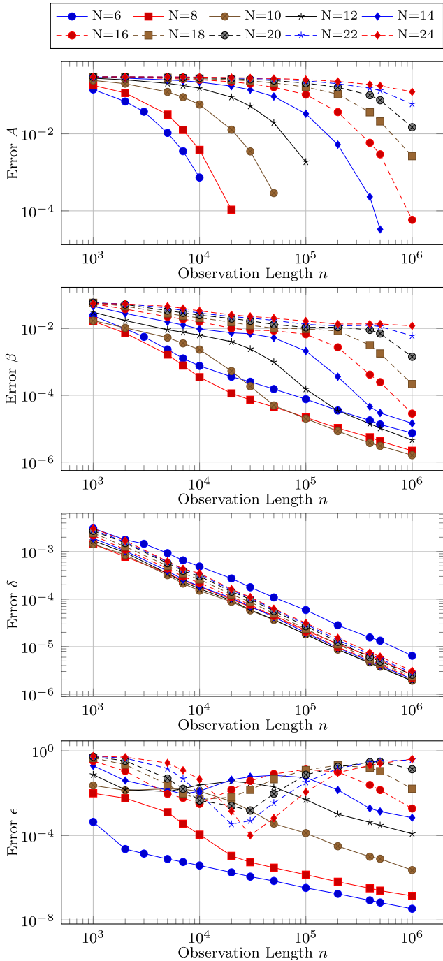
Fig. 4. Accuracy of reconstructed network and estimated parameters in dependency of the observation length n . Discontinued graphs in the first, logarithmically scaled plot refer to zero errors of the estimate of A .
