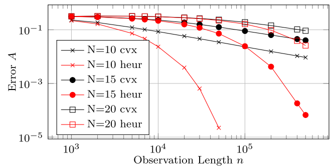
Fig. 3. Accuracy of the non-binary estimate A_{\text{cvx}} , given by (43), and the rounded estimate A_{\text{heur}} in dependency of the observation length n . Discontinued graphs in the logarithmically scaled plot refer to zero errors of the estimate of A .
