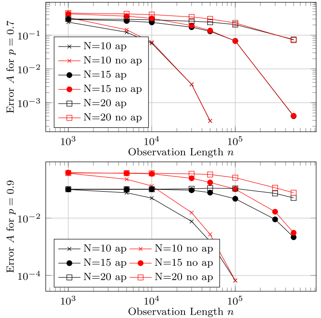
Fig. 9. Impact of a-priori knowledge: Comparison of accuracy of reconstructed network and estimated spreading parameters with a-priori knowledge (ap) and without a-priori knowledge (no ap) for the link probabilities p = 0.7 and p = 0.9 . Discontinued graphs in the logarithmically scaled plots refer to zero errors of the estimate of A .
