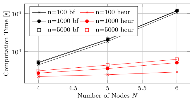
Fig. 2. Comparison of computation time of heuristic (heur) and brute-force (bf) approach in dependency of the number of nodes N .
