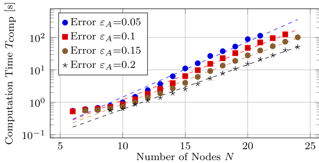
Fig. 11. Required computation time T_{\text{comp}} for given average fraction \varepsilon_A of erroneous links of the estimate of A , in dependency of the number of nodes N . The points are obtained by interpolation and the fitted subexponential dependencies are given by the dashed graphs.
