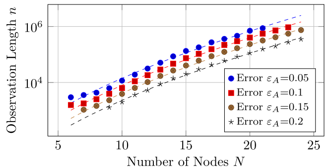
Fig. 10. Required observation length n for given average fraction \epsilon_A of erroneous links of the estimate of A , in dependency of the number of nodes N . The points are obtained by interpolation and the fitted subexponential dependencies are given by the dashed graphs.
