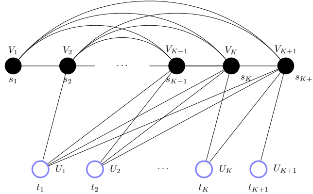
Figure 2: The partition of node set \mathcal{N} = V_1 \cup U_1 \cup V_2 \cup U_2 \cup \dots \cup V_K \cup U_K \cup V_{K+1} in a weighted threshold graph. Each nodal set V_i forms a clique of size s_i . Each nodal set U_i forms an empty graph of size t_i . The link between two sets indicates a complete bipartite connection, where every node in one set is connected to every node in the other set.
